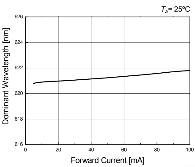
Forward Current vs. Dominant Wavelength
