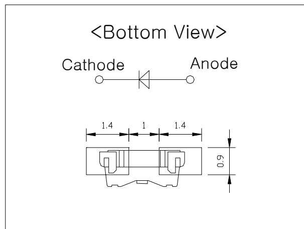
Recommended solder Pattern
